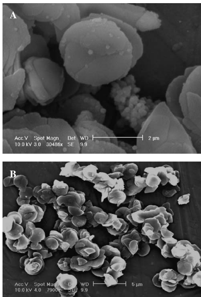
Fig. 4. Scanning electron microscopy pictures of HTlc-FER intercalation compounds (A) and blank HTlc-Cl matrix (B).
